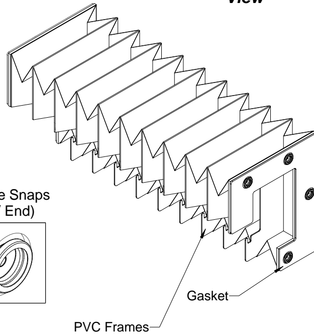
Isometric Rear View
